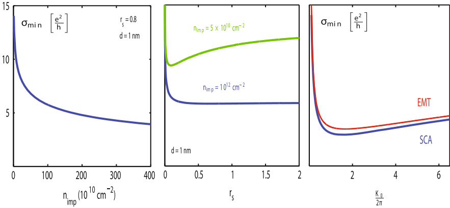
Fig. 12.9 Dependence of graphene minimum conductivity on disorder parameters. All panels have the same scale for \sigma_{\text{min}} on the y-axis. Left panel : For charged impurities, \sigma_{\text{min}} decreases monotonically as a function of impurity density. Center panel : Samples with large Coulomb disorder (blue curve) show almost no dependence of \sigma_{\text{min}} on the effective fine structure constant r_s ; cleaner samples (green curve) show the minimum conductivity increasing weakly with r_s . Right panel : For the Gaussian correlated impurity model, the effective medium theory result (12.32) is slightly larger (red curve) than the analytic result \sigma_{\text{min}}[x = K_0/2] = 2e^x/xI_1(x) shown in blue and derived from (12.30)
