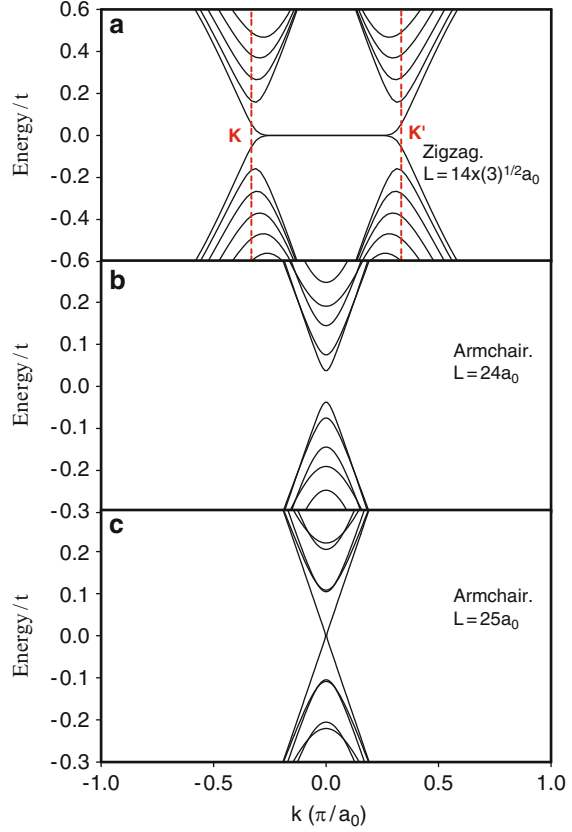
Fig. 10.2 Examples of energy bands for a graphene nanoribbon with periodic boundary conditions in one direction. k is the wavevector parallel to the nanoribbon edge, measured with respect to the center of the Brillouin center. (a) Ribbon terminated in zigzag edges with 56 atoms in the unit cell. The dispersionless states correspond to confined surface states. The band structures of insulating and metallic armchair nanoribbons are plotted in (b) and (c) respectively
