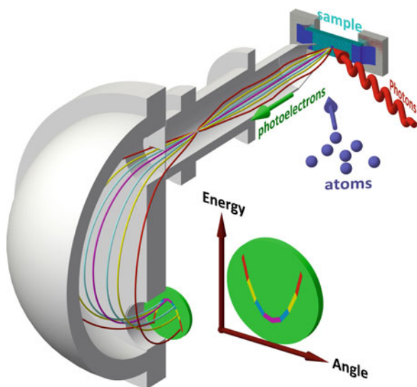
Fig. 4.1 Schematic diagram of the angle-resolved photoemission spectroscopy (ARPES) measurement of graphene. Incident UV or soft X-ray photons (wavy arrow) impinge on the graphene target, exciting photoelectrons with a distribution of angles and energies. A planar cut of this distribution is collected by an angular-imaging electron lens (shown in cross section) and dispersed by a nested set of hemispheres held at appropriate potentials. The energy-angle dispersion of the photoelectrons is mapped onto an imaging channel plate. By conducting experiments under a flux of atoms or other adsorbates, doping- and density-dependent studies can be accomplished
