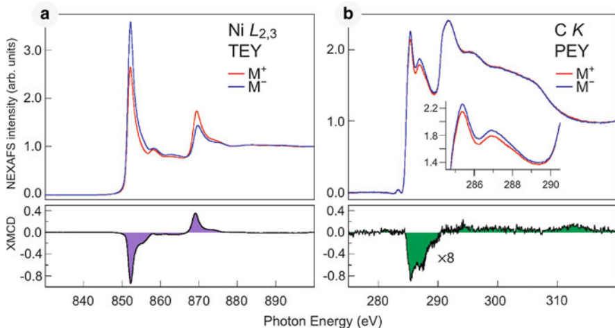
Fig. 7.12 XMCD spectra of the graphene/Ni(111) system measured at the Ni L_{2,3} (a) and C K absorption edges (b). The corresponding differences reflecting the strength of the dichroic signal are shown in the lower part of the respective figures. Data are taken from [75, 86]
