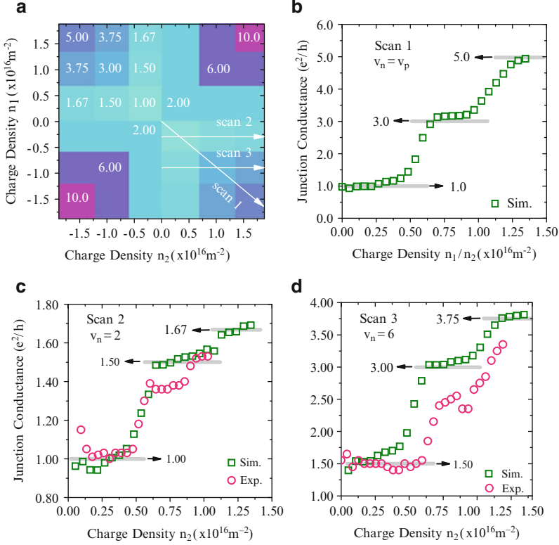
Fig. 15.12 (a) Depiction of the theoretical Ohmic plateaus \hat{\sigma}_{pn}(v_n, v_p) [55] as a function of n_1/n_2 , where the different colors represent the filling factors. (b)–(d) plots the linescan for the following cases: (1) v_n = v_p ; (2) v_n = 2 ; and (3) v_n = 6 , respectively; it also compares the simulation results with the experimental data. The experimental data are taken from [34] for a two-terminal pn junction quantum Hall measurement at B = 4 T. The simulations are done at B = 10 T. In the experimental data, the gate oxide capacitance is used as a fitting parameter. (Fig. is adapted from [56])
