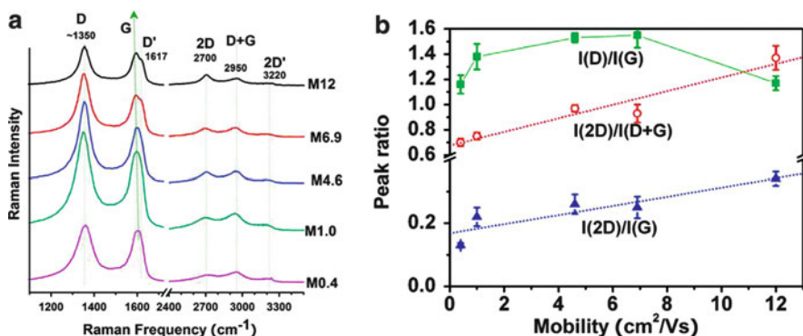
Fig. 14.10 (a) Raman spectra for five selected transistor devices with various values of effective mobility. The labels M0.4, M1.0, M4.6, M6.9, and M12 represent the devices with mobility 0.4, 1.0, 4.6, 6.9, and 12 \text{cm}^2/(\text{V s}) , respectively. (b) Various ratios for the integrated peak area for D, G, 2D, and D+G bands. Reprinted with permission from [94]. Copyright 2009 American Chemical Society
