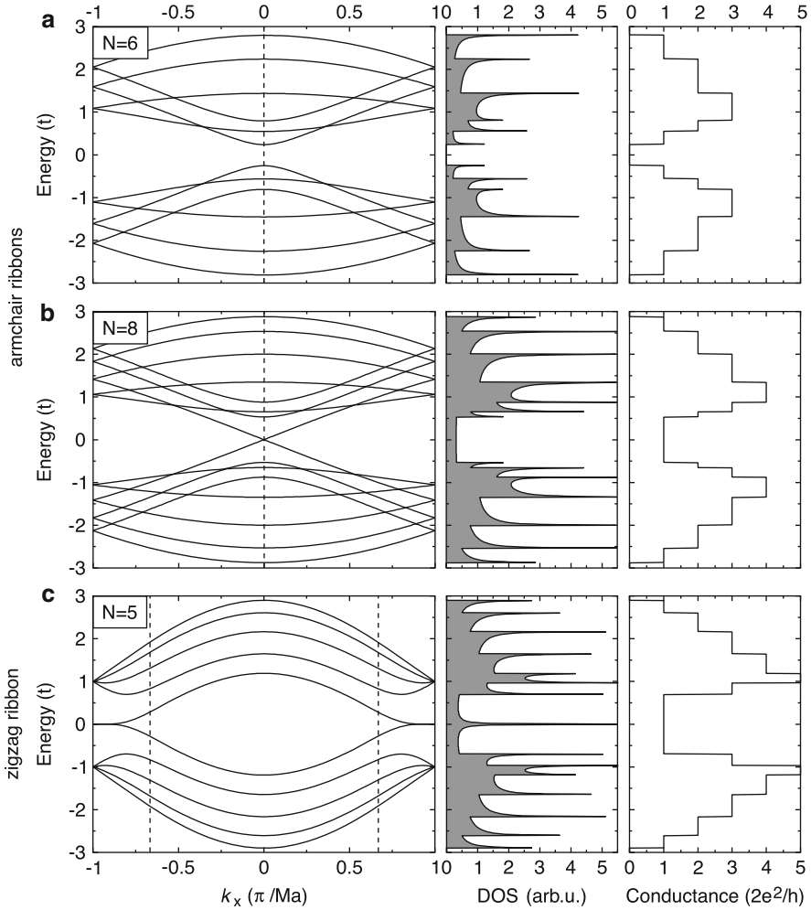
Fig. 13.2 The dispersion relation ( left column ), DOS ( middle column ), and conductance ( right column ) for ideal armchair (a), (b), and zigzag (c) graphene ribbons. The dashed vertical lines in the dispersion plots show the Dirac point location of 2D graphene projected onto the longitudinal axis of the ribbon. Ma is the unit cell size of the ribbon: M = 3 for armchair and M = \sqrt{3} for zigzag ribbons; a = 0.142 nm. The Dirac point corresponds to zero energy
