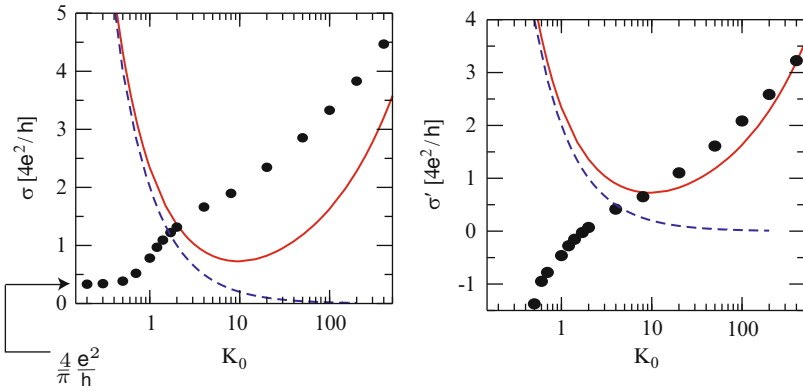
Fig. 12.12 Comparison of graphene conductivity calculated using the fully quantum theory and the semiclassical self-consistent approximation. The data points are the Landauer result (see [41]), while the solid red line is the SCA result (12.30). The dashed blue line is the Boltzmann result which for this model has a minimum conductivity that scales as K_0^{-1} (see (12.18)). For vanishing disorder, the quantum results give the universal value \sigma_{\min} = 4e^2/\pi h . With increasing disorder, the quantum results first increase sharply at K_0 \approx 1 followed by a more gradual increase for K_0 \gtrsim 10 (left panel). To test whether this gradual increase is compatible with the self-consistent approximation, in the right panel we plot the classical component of the Landauer conductivity \sigma' = \lim_{L \rightarrow \infty} [\sigma(L) - \pi^{-1} \ln(L/\xi)] , where we have verified that for \sigma \gtrsim 4e^2/h the L dependence is consistent with weak antilocalization. The fully quantum result agrees with the self-consistent approach when the number of electrons per puddle N_e \approx \pi n^* \xi^2 = K_0/2\pi \gtrsim 1.6
