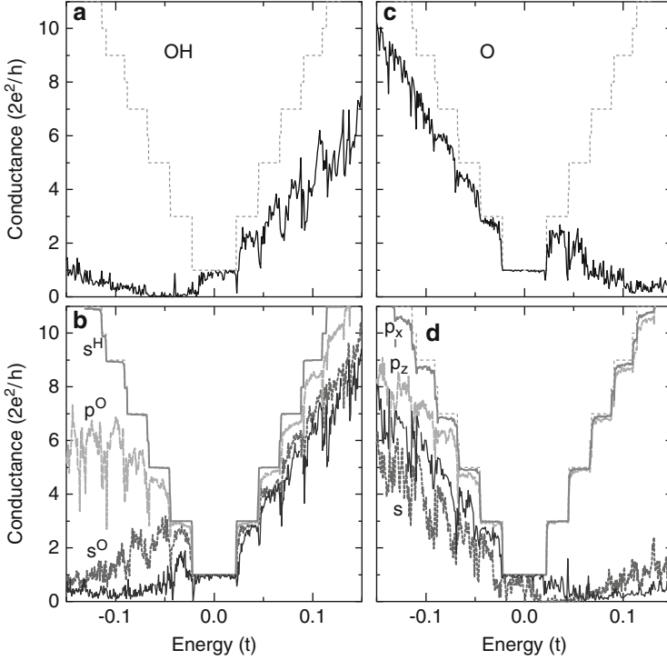
Fig. 13.14 The conductances ( solid black lines ) vs. Fermi energy for ribbons with adsorbed OH ((a), (b)) and O ((c), (d)) at concentrations p = 10^{-4} . The geometries of the adsorbates and graphene are shown in Fig. 13.10. (a) and (c) include the effects of the local rehybridization of the graphene from sp^2 to sp^3 bonding embodied in Table 13.2. (b) and (d) do not include rehybridization and are based on Table 13.3. Thin dotted pale grey lines show the conductance of the ideal ribbon with no defects. The other grey lines in (b) and (d) show the effects on the conductance of individual valence orbitals of the adsorbed species. Ribbon width W = 30 nm; length L = 500 nm. Temperature T = 0 . t = 2.7 eV. The Dirac point is at zero energy. Adapted from [55]
