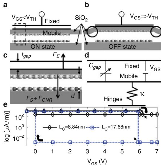
Fig. 16.8 The side-view schematics of the bilayer ZGNR NEM switch at (a) ON-state and (b) OFF-state. A free-body diagram of the dashed box region in (a) is shown in (c) and the equivalent circuit used to analysis the device is shown in (d). The device characteristics with different channel lengths are shown in (e)
