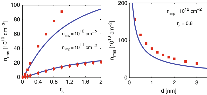
Fig. 12.5 Dependence of the carrier density fluctuations on effective fine structure constant r_s ( left panel ) and distance of the Coulomb impurities from the graphene sheet d ( right panel ). Solid lines are the self-consistent result (12.20) and data points were computed in [32] using a density functional approach
