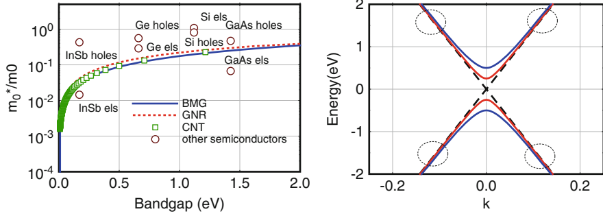
Fig. 18.9 Scaling of graphite effective masses shows that increasing the bandgap increases the mass m^* = p_F/v_F due to the decrease in average curvature arising from a pinning of the E–k at high-energy values [19]
