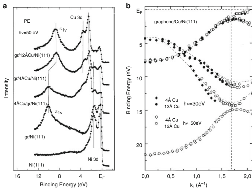
Fig. 7.21 (a) Normal emission PE spectra demonstrating the process of 3d metal intercalation underneath graphene layer on Ni(111): of the clean Ni(111) surface, a graphene/Ni(111), 4 Å Cu/graphene/Ni(111), as well as the graphene/4 Å Cu/Ni(111) and the graphene/12 Å Cu/Ni(111) systems. (b) Experimental band structure of the graphene/Cu/Ni(111) system. For comparison, the band structure of pristine graphite is shown by dashed lines. Data are taken from [23]
