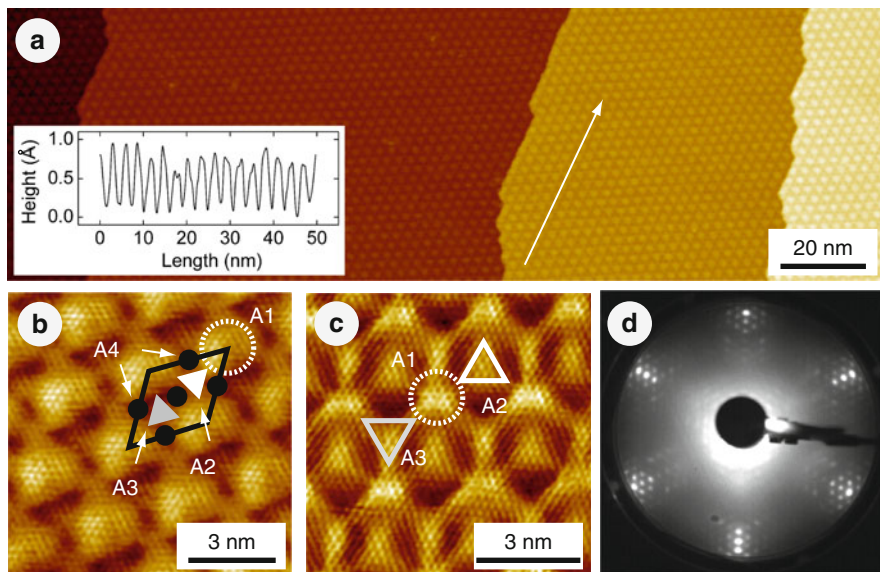
Fig. 7.16 (a) Large-scale STM image of an epitaxial graphene layer on the Rh(111) surface. Inset shows a height profile measured along the white arrow. (b) High magnification image of the unit cell of the moiré structure. The black rhombus outlines the supercell of the moiré structure. Main surface features are marked in the image: moiré maximum (A1) by a circle, the brighter half-cell (A2) by a white solid triangle, the darker half-cell (A3) by a gray solid triangle, and bridging black minima (A4) by black solid circles. (c) Atomically resolved STM image of the moiré structure of the graphene layer on Rh(111) taken with different tunneling parameters compared with (b). (d) LEED image of the graphene layer on Rh(111) taken at a primary electron energy of 58 eV. Tunneling parameters for STM images: (a) U_T = 1.12 V; I_T = 0.18 nA; (b) U_T = 0.01 V; I_T = 2.56 nA; (c) U_T = 0.02 V; I_T = 30 nA. Data are taken from [117]
