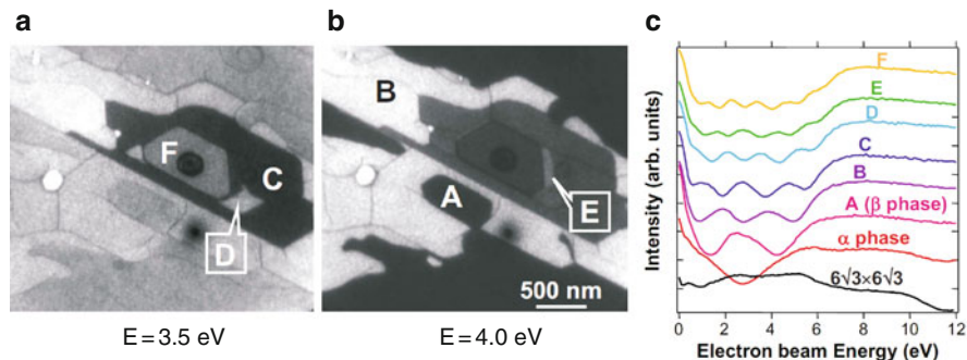
Fig. 5.7 LEEM images of graphene layers grown on SiC(0001) recorded at electron energies of (a) 3.5 eV and (b) 4.0 eV. The image contrast is caused by a thickness-dependent reflectivity. (c) Reflectivity as a function of electron energy for the regions marked in (a) and (b). The analysis led to the conclusion that the number of minima in the reflectivity spectrum corresponds to the number of graphene layers: \alpha : 1 monolayer; A: 2 monolayers, B: 3 monolayers, etc. Reprinted with permission from [86]. Copyright (2008) by the American Physical Society
