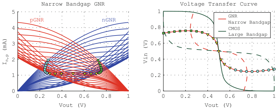
Fig. 18.21 Comparison of VTC curves for narrow bandgap GNR and 45 nm CMOS technology. Narrow bandgap GNRFETs will be more susceptible to noise than CMOS due to smaller noise margins. An possible design metric would be to limit the supply voltage to V_{dd} < 0.8/W , where W is the width of the semiconducting GNR channel
