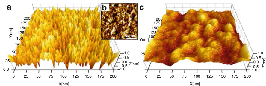
Fig. 3.13 (a, b) 3D and 2D constant current STM image of monolayer graphene. (c) 3D tapping mode AFM image of the \text{SiO}_2 substrate (Reprinted figure with permission from [27]. Copyright (2009) by the American Physical Society)
