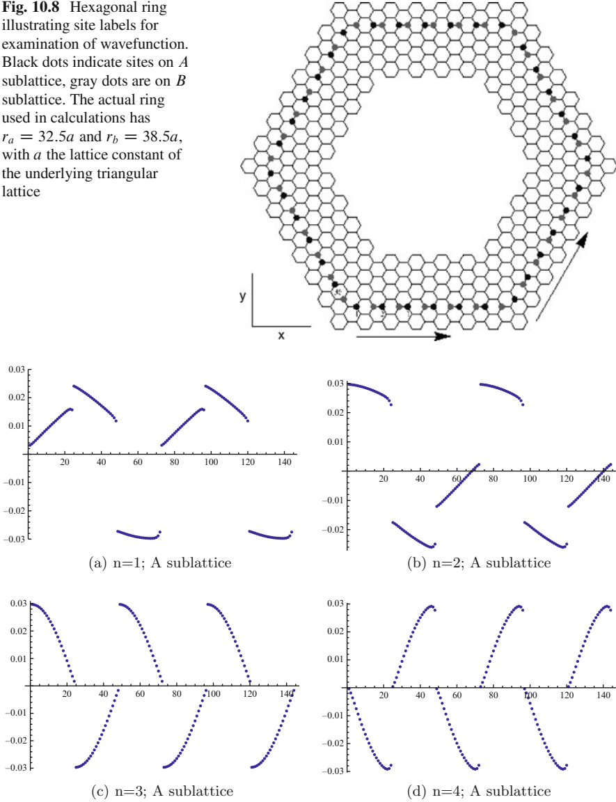
Fig. 10.9 Wavefunctions at zero flux \Phi for the four lowest eigenstates n = 1, 2, 3, 4 illustrated in Fig. 10.7b
