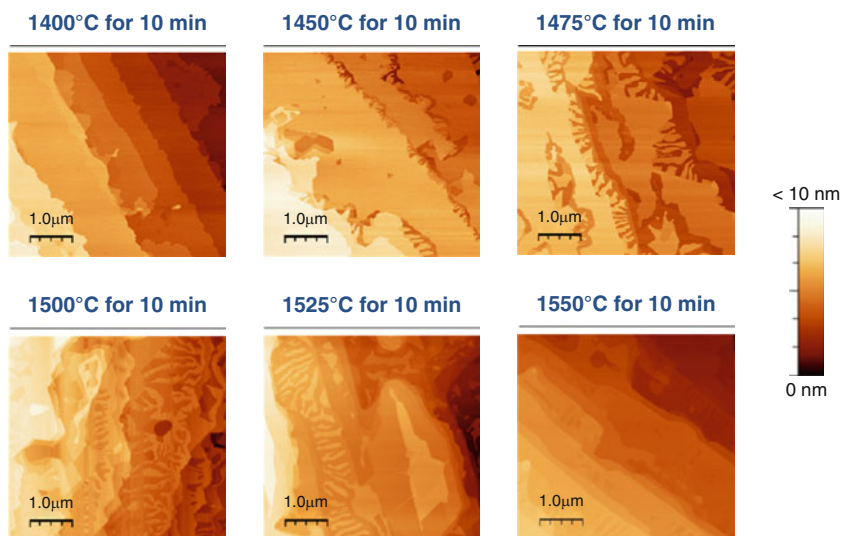
Fig. 6.2 AFM profilometry micrographs of Si-face SiC substrates after H 2 etching and thermal decomposition at 1,400°C, 1,450°C, 1,475°C, 1,500°C, 1,525°C, and 1,550°C for 10 min in vacuum (low- 10^{-5} mbar)
