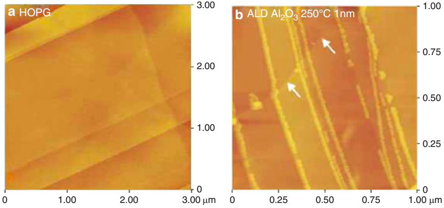
Fig. 6.6 (a) AFM images of HOPG surface with graphene terraces and (b) similar surface after 1 nm thick ALD \text{Al}_2\text{O}_3 growth
