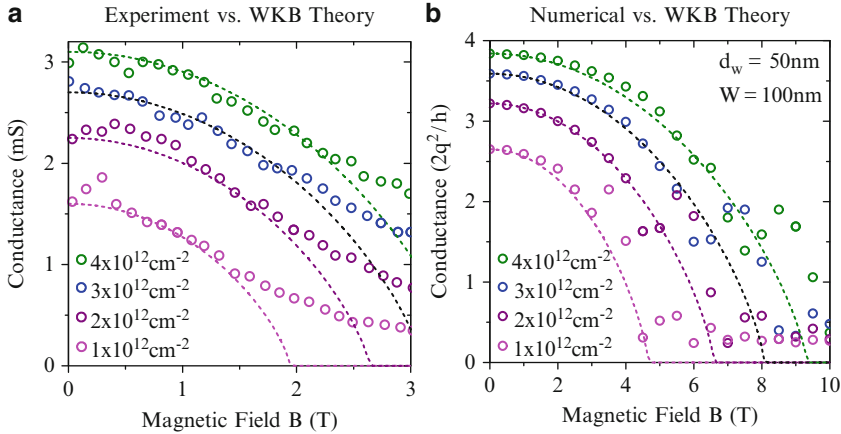
Fig. 15.7 (a) Experimentally measured (2R_{n1}^{\text{odd}})^{-1} of a symmetric pn junction, i.e., n_1 = -n_2 , at various concentrations n_1 , shown in symbols. The dashed lines are the results computed from (15.42), where \mathcal{G}_{np}^0 is used as a fitting parameter for each case (see text). The pn transition widths for each curve are assumed to be 120 nm, 125 nm, 130 nm and 135 nm for increasing values of n_1 . (b) Numerically simulated \mathcal{G}_{np} at various concentrations n_1 , shown in symbols. The dashed lines are again the results computed from (15.42)
