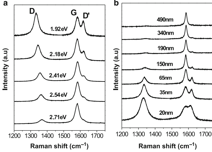
Fig. 2.7 The Raman spectra of (a) a nanographite sample heat treated at 2,000°C ( L_a = 35 nm), for five different laser excitation energies (1.92 eV, 2.18 eV, 2.41 eV, 2.54 eV, and 2.71 eV). (b) Nanographite samples with different crystallite sizes L_a using 1.92 eV laser excitation energy [40]
