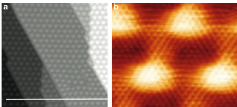
Fig. 7.15 (a) 500 \text{ Å} \times 500 \text{ Å} topographic STM image recorded after annealing Ru(0001) sample at 1,470 K. The surface is fully covered by graphene and Ru step edges are aligned along the main directions of the overlayer, indicating a restructuring of the underlying Ru surface. (b) 50 \text{ Å} \times 50 \text{ Å} atomically resolved image of the graphene overlayer on Ru(0001). The image shows three different levels of apparent heights, namely four bright maxima, a dark minimum in the center between the three maxima on the right hand side, and a less dark minimum between the three maxima on the left hand side. Tunneling parameters for STM images: (a) I_T = 1 \text{ nA} , U_T = -0.2 \text{ V} ; (b) I_T = 1 \text{ nA} , U_T = -0.05 \text{ V} . Data are taken from [42]
