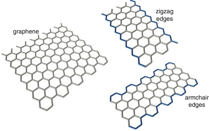
Fig. 2.2 Zigzag and armchair edges in monolayer graphene nanoribbons. The geometrical edge structure and the number of atomic rows of carbon atoms normal to the ribbon axis determine the electronic structure and ribbon properties (Images courtesy of M. Hofmann, MIT.)
