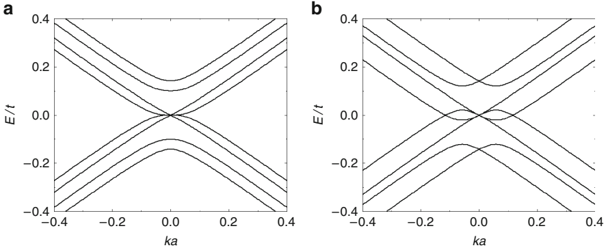
Fig. 11.16 Energy band structure near the K point for (a) ABCB-stacked and (b) ABBC-stacked tetralayer graphene with t = 3 \text{ eV} and t_{\perp} = 0.1t
