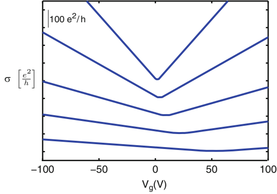
Fig. 12.13 Summary of theoretical predictions of the self-consistent approximation. Curves ( from top to bottom ) are for impurity density n_{\text{imp}} = [20, 40, 80, 160, 320] \times 10^{10} \text{ cm}^{-2} and are offset by 100 e^2/h for clarity. The self-consistent theory [14] predicts that for charged impurity scattering, cleaner samples have (1) higher mobility, (2) narrower minimum conductivity plateaus, (3) smaller Dirac point offsets, and (4) larger values for the minimum conductivity
