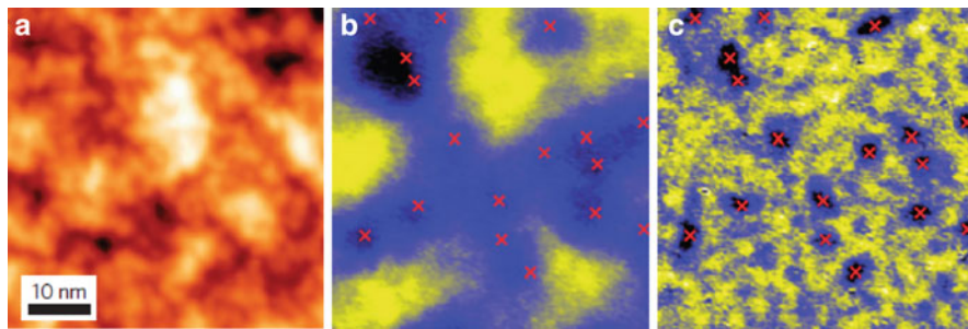
Fig. 3.16 (a) STM topography of graphene on SiO 2 . (b) dI/dV map at a bias near the Dirac point showing electron puddles due to charge fluctuations over the same region of graphene as (a). Red crosses indicate the location of quasiparticle scattering centers observed in (c). (c) dI/dV map of the same area at larger bias revealing impurity scattering centers in electron-rich charge-density puddles (red crosses) (Reprinted by permission from Macmillan Publishers Ltd: Nature Physics [26], copyright (2009).)
