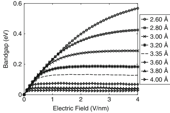
Fig. 17.8 Band gap modulation of strained bilayer with an external electric field. The dashed line is for equilibrium c = 3.35 Å, for which band gap saturates at about 0.13 eV. A convex relation is observed as a function of electric field above c \approx 2.5 Å. By decreasing c , band gap modulation increases due to increased interlayer hopping
