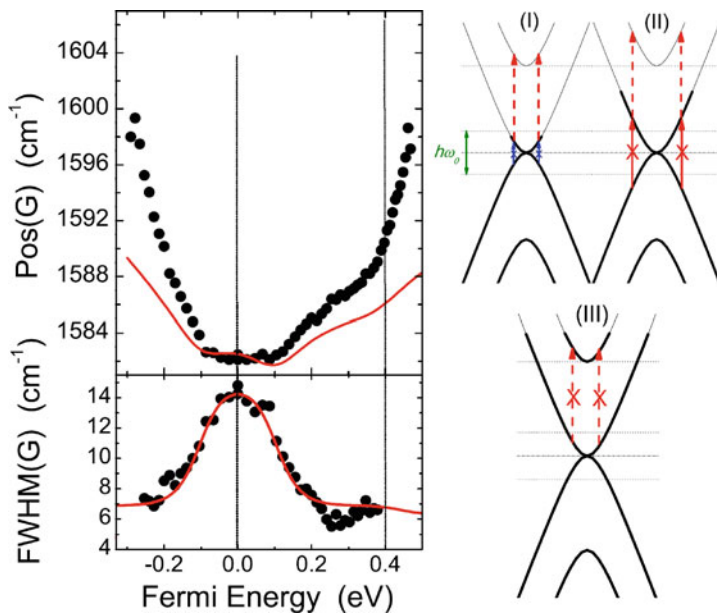
Fig. 2.18 Position of the peak frequency [Pos(G)] and the linewidth [FWHM(G)] measured at full width half maximum intensity for the Raman G -band feature of doped bilayer graphene. Black circles : measurements; thin line : finite-temperature nonadiabatic calculation. On the right , schematics of the electron–phonon coupling at three different doping levels, as indicated by the thicker lines on the electronic bands (Adapted from [73].)
