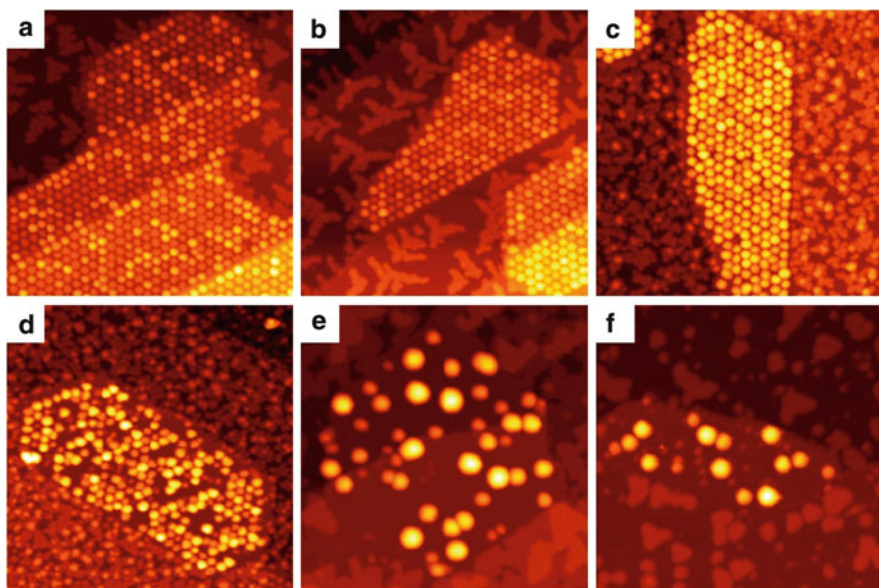
Fig. 7.23 700 \text{ \AA} \times 700 \text{ \AA} STM images of the Ir(111) surface covered by graphene flakes after the deposition of various metals at 300 K. (a) 0.20 ML Ir, average cluster size S_{\text{av}} = 17 atoms; (b) 0.25 ML Pt, S_{\text{av}} = 22 atoms; (c) 0.44 ML W, S_{\text{av}} = 38 atoms; (d) 0.53 ML Re, S_{\text{av}} = 60 atoms; (e) 0.77 ML Fe, S_{\text{av}} = 420 atoms; (f) 0.25 ML Au, S_{\text{av}} = 100 atoms. Data are taken from [144].
