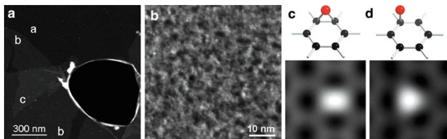
Fig. 14.6 (a, b) ADF-STEM image of the graphene oxide films where mono-, bi- and trilayers are labeled as a , b , and c , respectively. Round opening in the middle is a hole through the single film. (c, d) Simulated ADF-STEM images of graphene with oxygen bonded to the honeycomb of the graphene. The ball-stick models at the top illustrate the structures. Reprinted with permission from [71]. Copyright 2009 American Chemical Society
