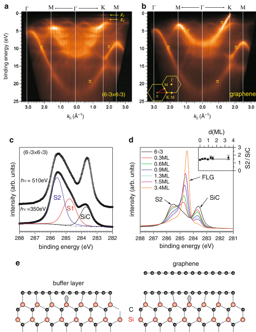
Fig. 5.4 (a) and (b) Photoelectron intensity map vs. binding energy and parallel electron momentum of SiC(0001)-(6 \sqrt{3} \times 6\sqrt{3} )R30° and a sample with one monolayer graphene, respectively. The sketch in (b) shows the direction of k_{\parallel} within the hexagonal Brillouin zone of graphene. (c) C1s core level spectra of the (6 \sqrt{3} \times 6\sqrt{3} )R30° reconstruction measured with two different photon energies. Also shown is a curve fit using three Voigt profiles. (d) C1s core level spectra of the (6 \sqrt{3} \times 6\sqrt{3} )R30° reconstruction and after growth of graphene. The inset shows the ratio between the intensity of component S2 and the SiC bulk component obtained by curve fitting. Adapted from [34]. (e) Model of the buffer layer, i.e. the (6 \sqrt{3} \times 6\sqrt{3} )R30° reconstruction, and of a monolayer of graphene on top of the buffer layer
