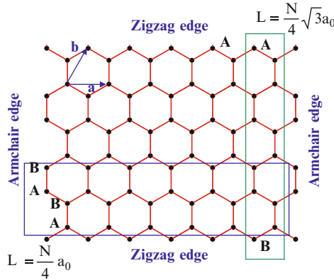
Fig. 10.1 The lattice structure of a graphene sheet. The primitive lattice vectors are denoted by \mathbf{a} and \mathbf{b} . Top and bottom are zigzag edges, left and right are armchair edges. Atoms enclosed in the vertical (horizontal) rectangle represent the unit cell used in the calculation of nanoribbons with zigzag (armchair) edges. The length of the nanoribbons, L , as function of the number of atoms, N , in the unit cell is also indicated
